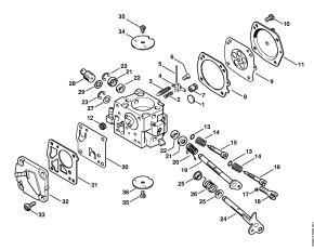
Carburetor HS-277
