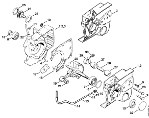
Crankcase
