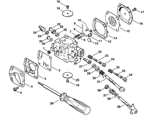
Carburetor HS-280, HS-281
