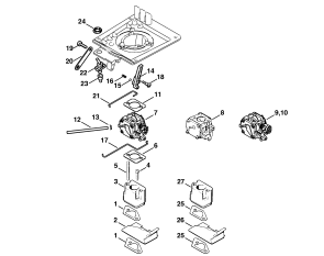
Throttle control
