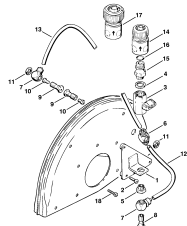
Water attachment (38.1995)
