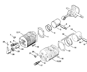
Cylinder
