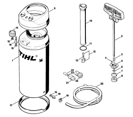
Pressurized water tank (23.96)
