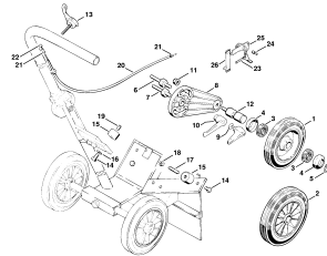
Stop depth wheel, Cart for cutquik
