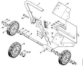
Cutquik cart, Splash guard
