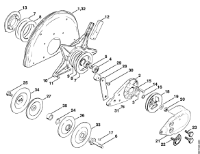
Support with guard (38.1995)
