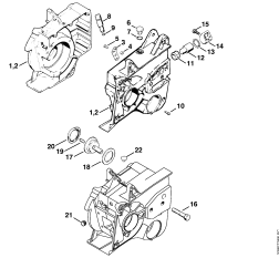
Crankcase → X 23 529 742, X 23 531 439 (27.91)
