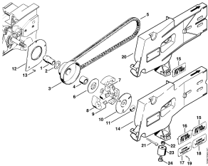
Coupling, Cast arm
