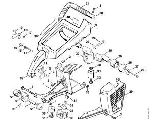
Shroud, Handle frame
