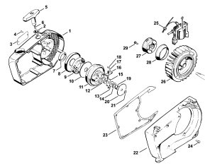
Rewind starter friction shoe → X 6 745 960 (30.80)
