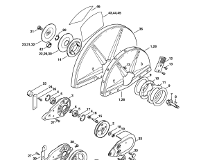
Support with guard
